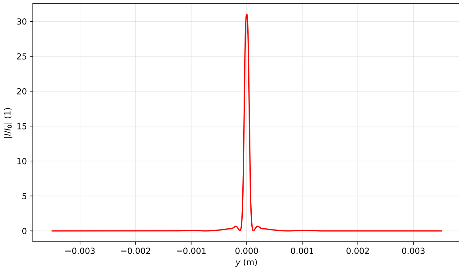
Intensity profile I(x=0, y, z=1.433)/I_0 , P_{in}=3.5P_{cr} , artificial time
